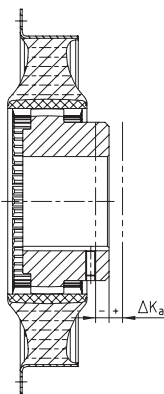
Axial displacement
